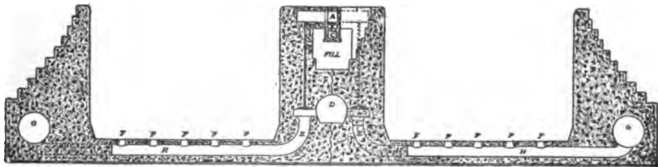
CROSS SECTION OF LOCK CHAMBER AND WALLS OR LOCKS
